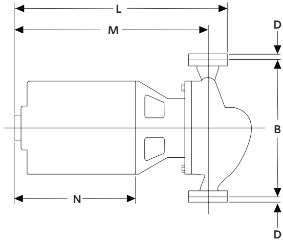
RIGID MOUNT
